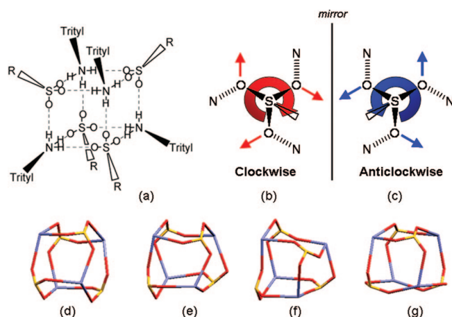
FIGURE 10. [4 + 4] Ion-pair clusters of triphenylmethylenamine 21 and organic sulfonic acids (a). Vortex-like hydrogen-bonding networks with clockwise (b) and anticlockwise (c) directions. Hydrogen-bonding networks of the clusters with 23 (4:0) (d), 25 (4:0) (e), 22 (3:1) (f), and camphorsulfonic acid (2:2) (g). The ratios of clockwise to anticlockwise directions are indicated in parentheses.
