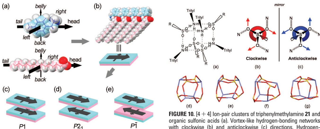
FIGURE 9. Hierarchical interpretation of chiral crystals from achiral molecules. Chiral conformers (a), chiral layers composed of the chiral conformers (b), chiral P1 crystal composed of the chiral layers stacked in a parallel fashion (c), chiral P2_1 crystal in an antiparallel fashion (d), and achiral P\bar{1} crystal in the reversed stacking (e).
